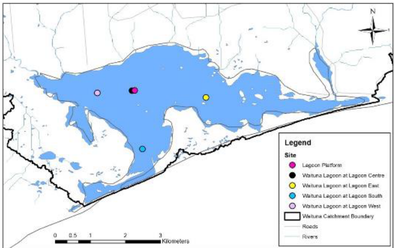
Figure 4-6: Waituna Lagoon Water Quality Monitoring Locations
