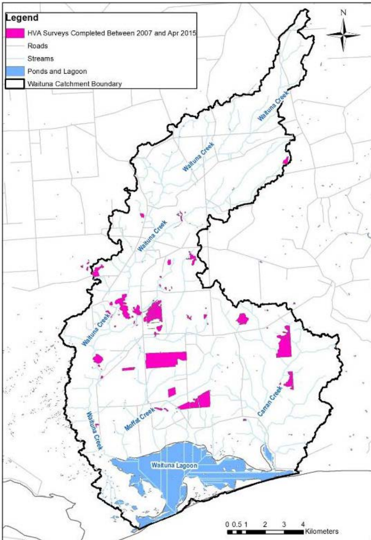
Figure 6-3: Location of HVA Surveys undertaken in Waituna Catchment
