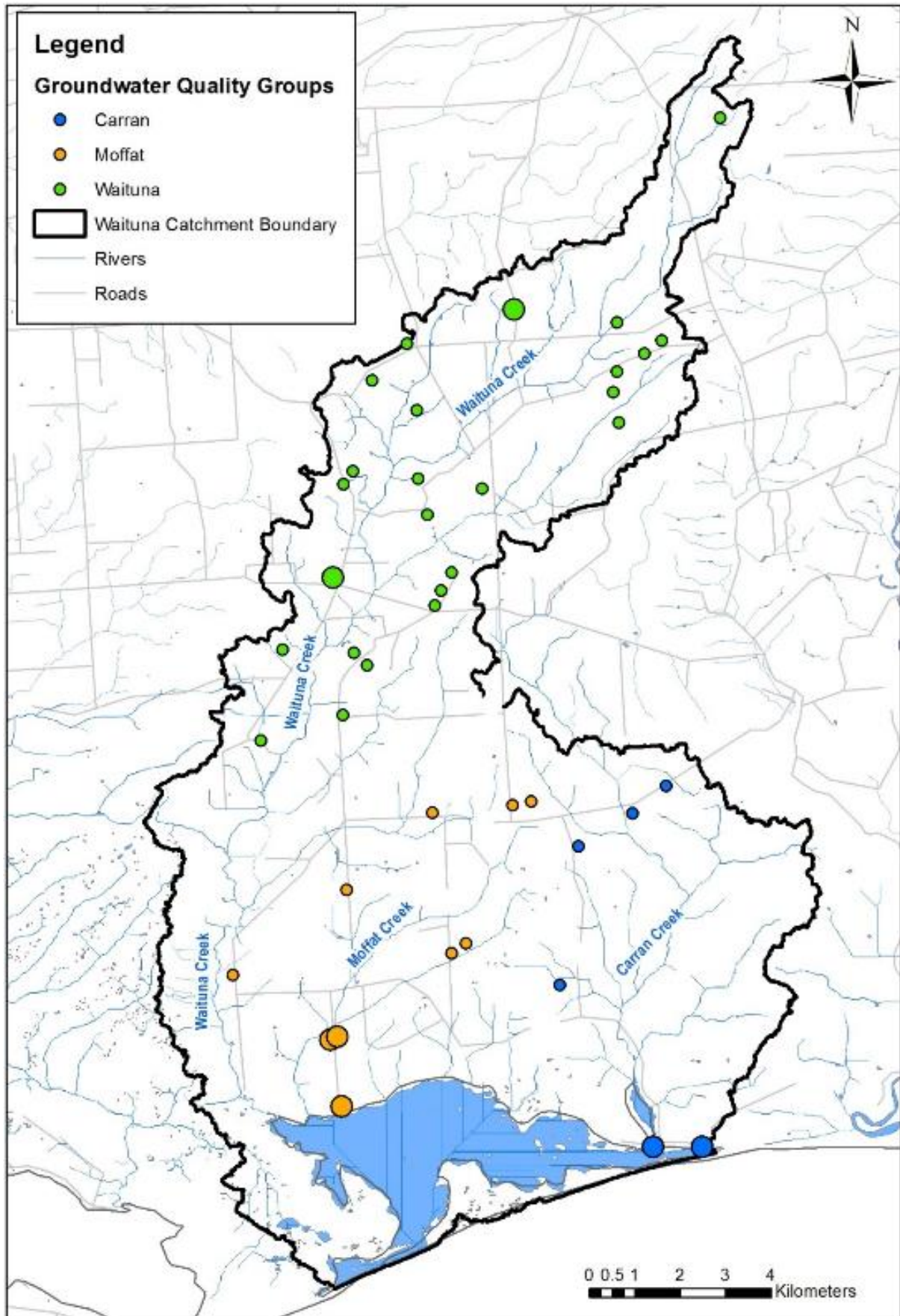
Figure 4-3: Groundwater monitoring sites grouped by catchment location
