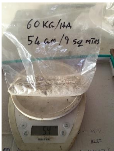
Confirming the calibration of the FPA spreading truck
